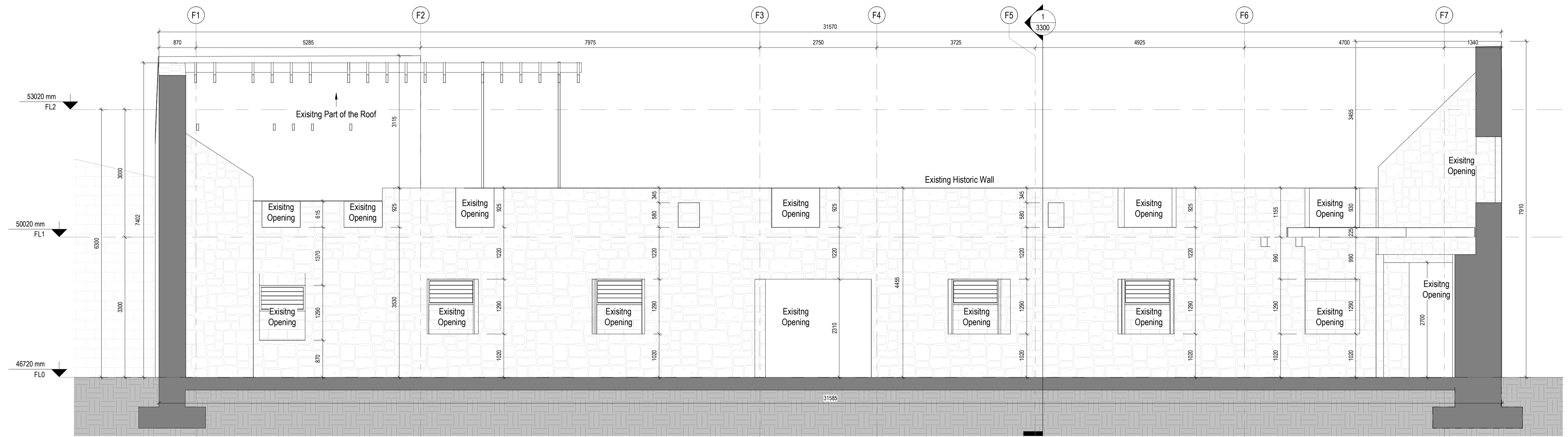
2 Existing Section North South Scale: 1 : 50
