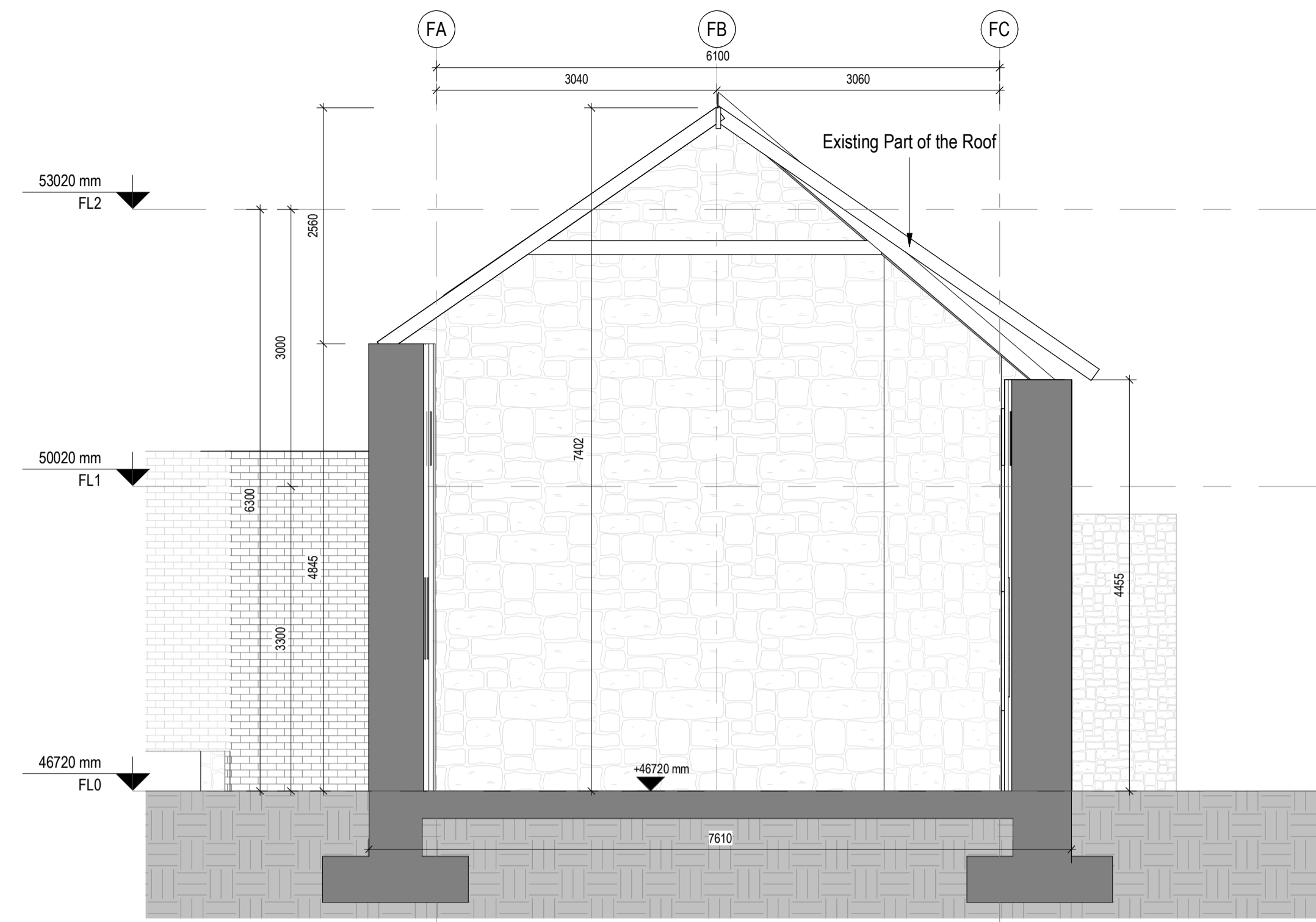
1 Existing Section East West Scale: 1 : 50
